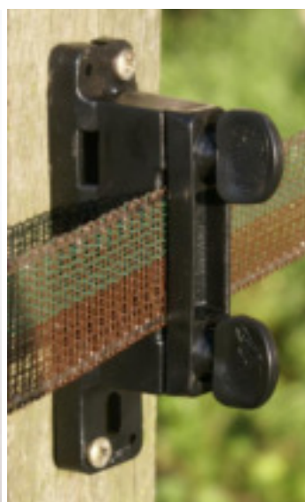
#8bl with 2 screws on wood
